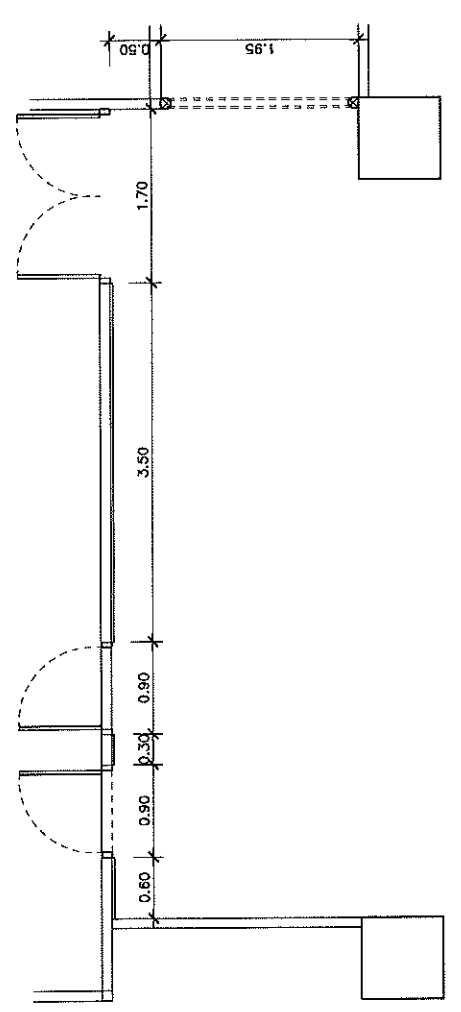
D KEYPLAN SCALE 1:1.50
